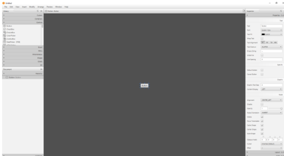
Figure 1: Button added
