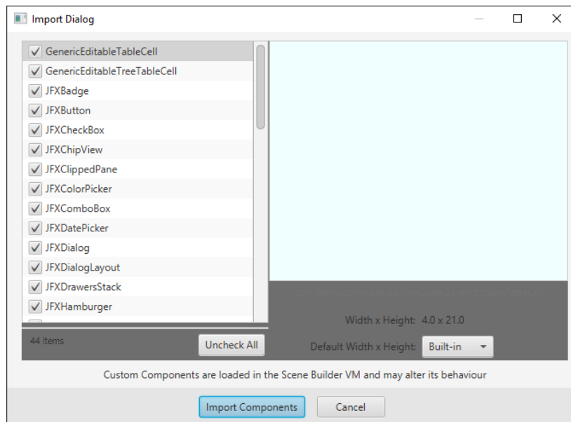
Figure 14: Import Dialog
