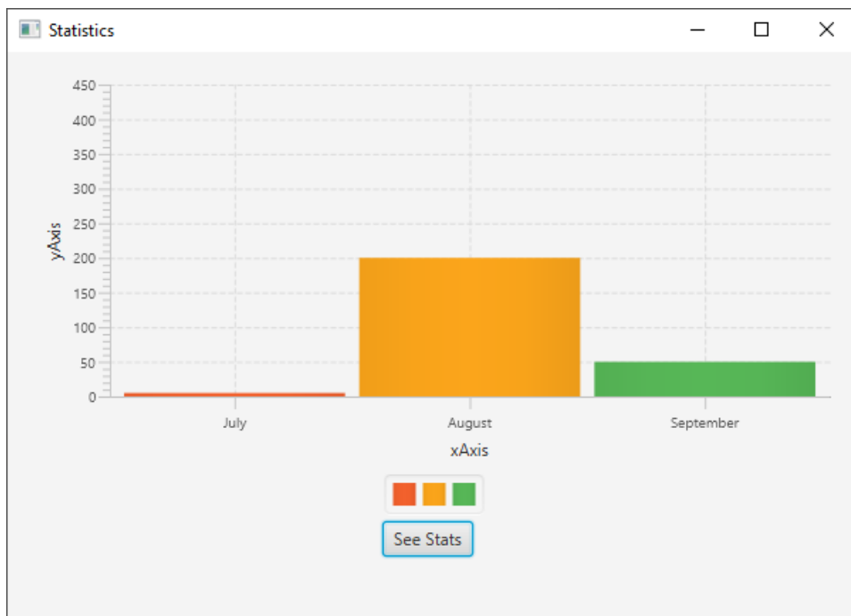
Figure 17: Open BarChart
