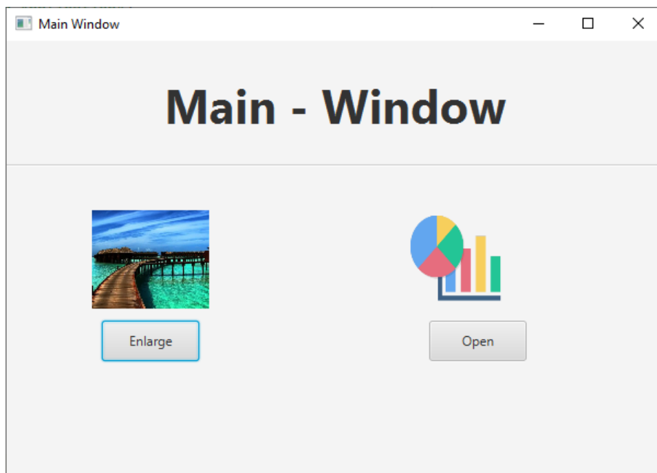
Figure 15: Main Window
