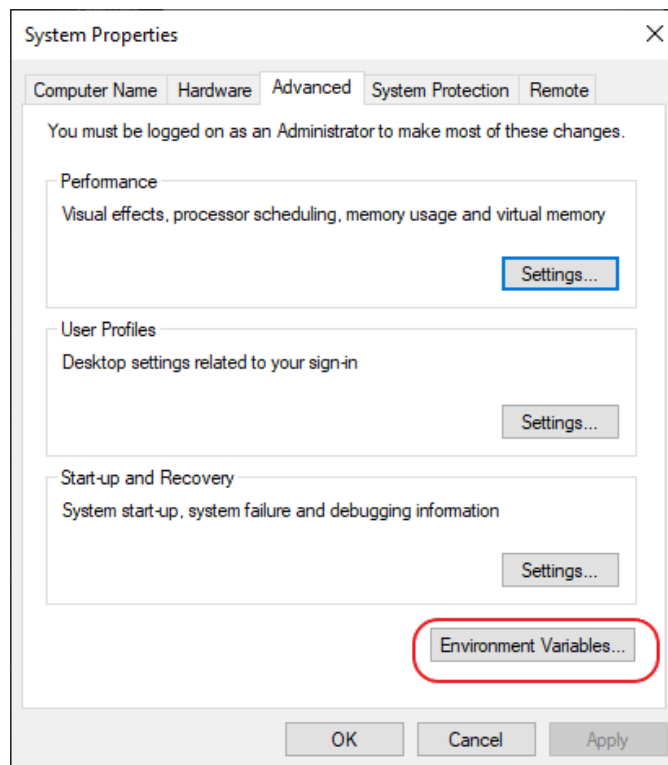
Figure 7: Environment Variable
